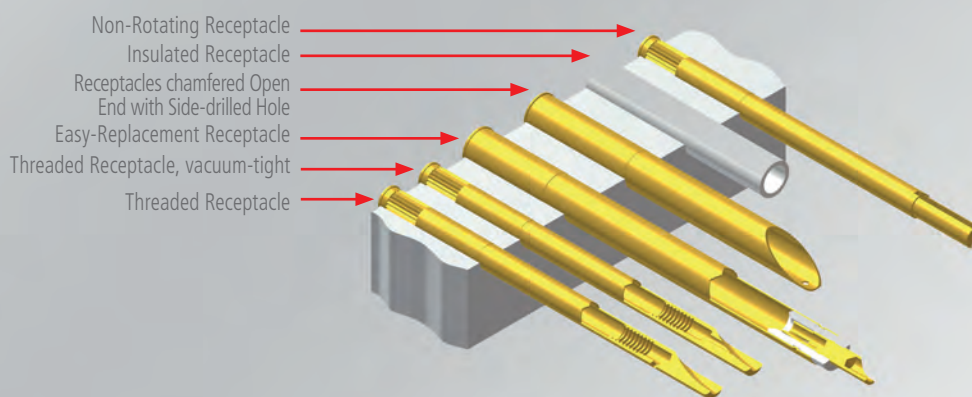
Fig. 2: Individual Types of Receptacles
